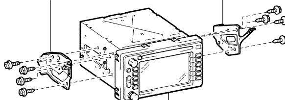
Radio Bracket No.2
