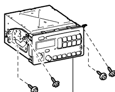
Radio Receiver Assembly W/bracket
