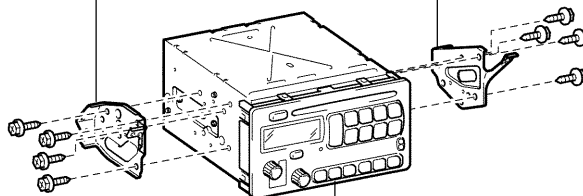
Radio Bracket No.2
